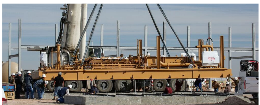
Caterpillar 3616/Ariel JGZ-4 Inlet Compressor Skids Being Lowered onto Existing Foundations
